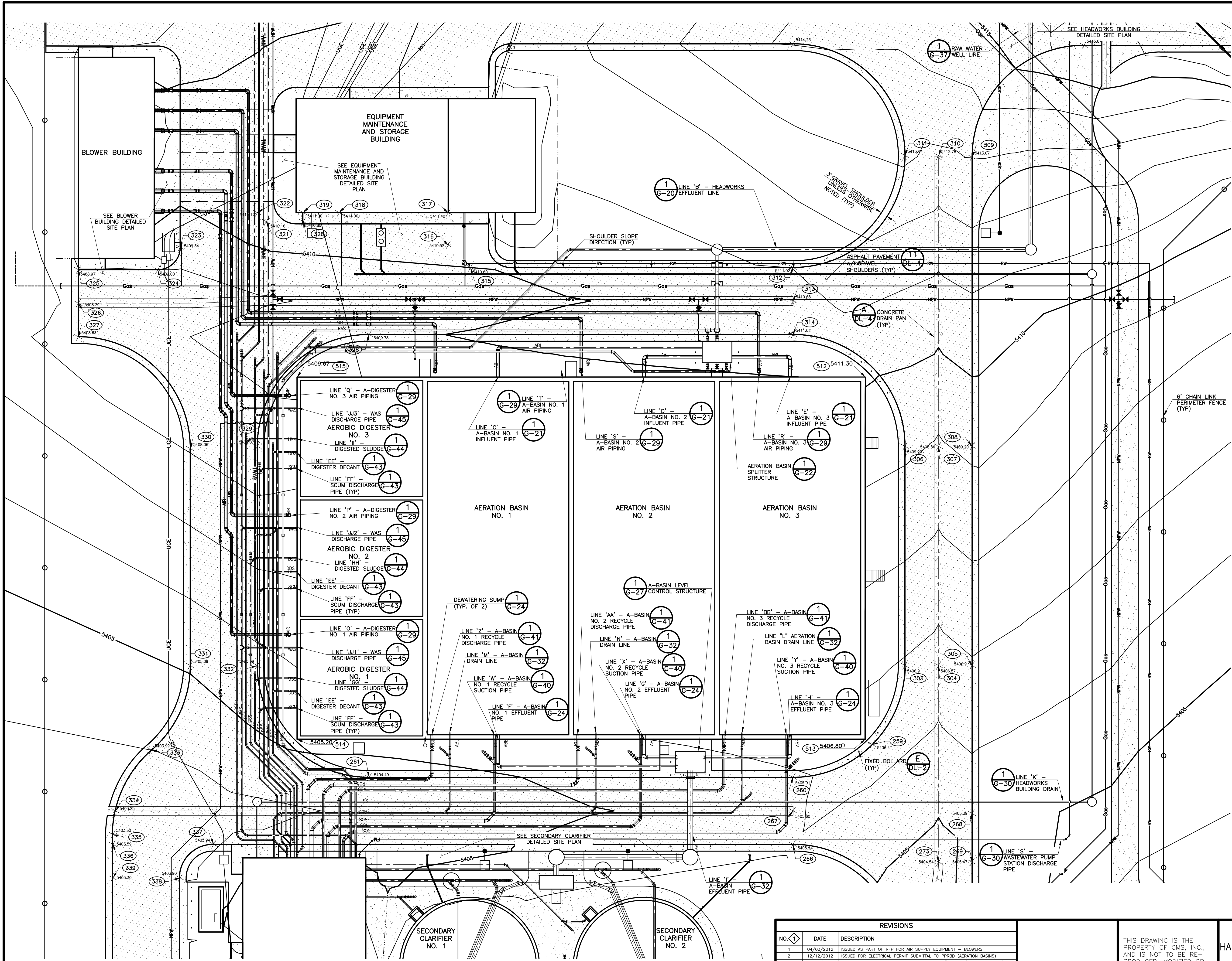
1 AERATION BASIN DETAILED SITE PLAN AB-10 SCALE: 1" = 20'
