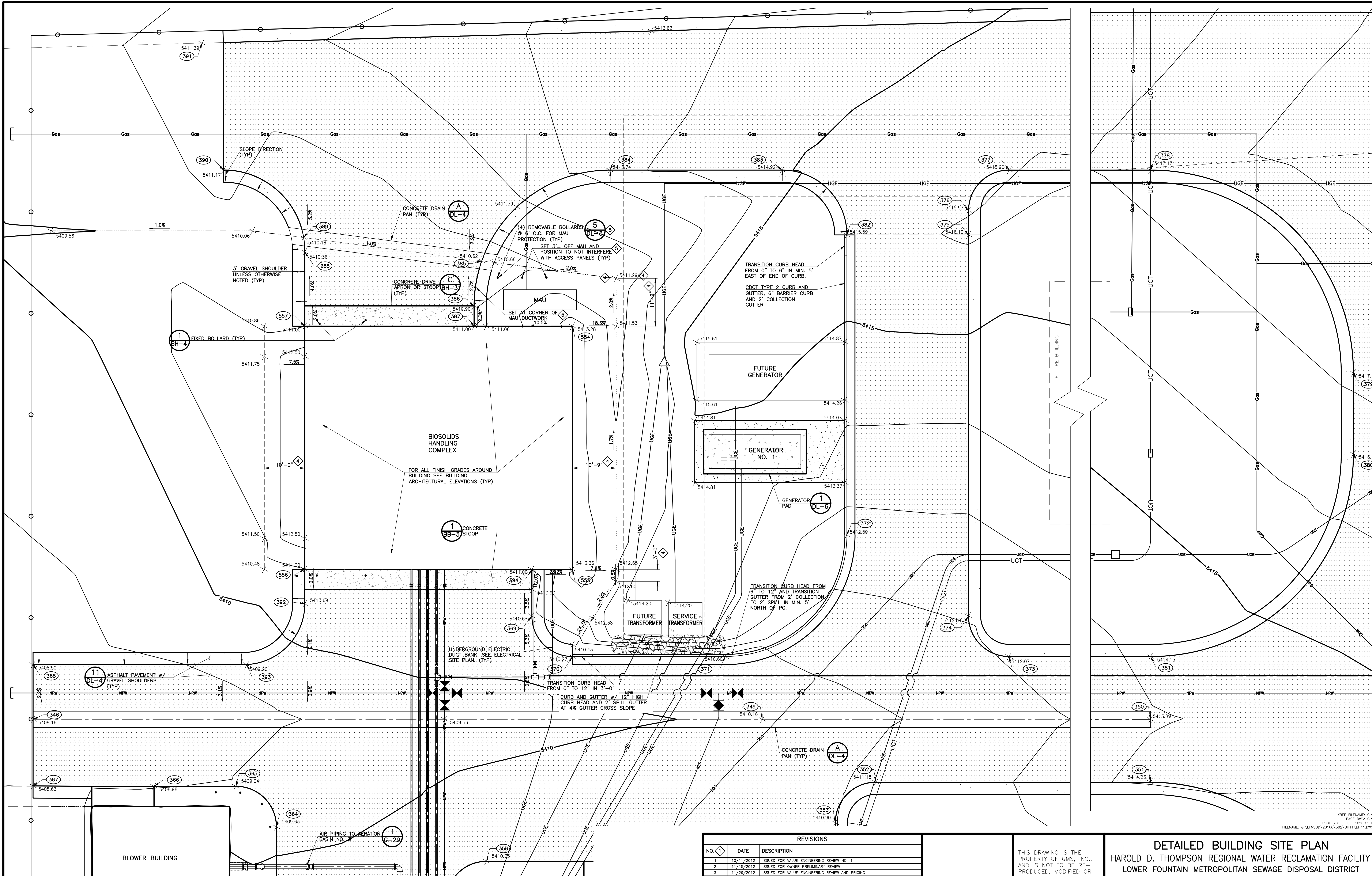
1 BIOSOLIDS HANDLING COMPLEX DETAILED SITE PLAN BH-11 SCALE: 1" = 10'
