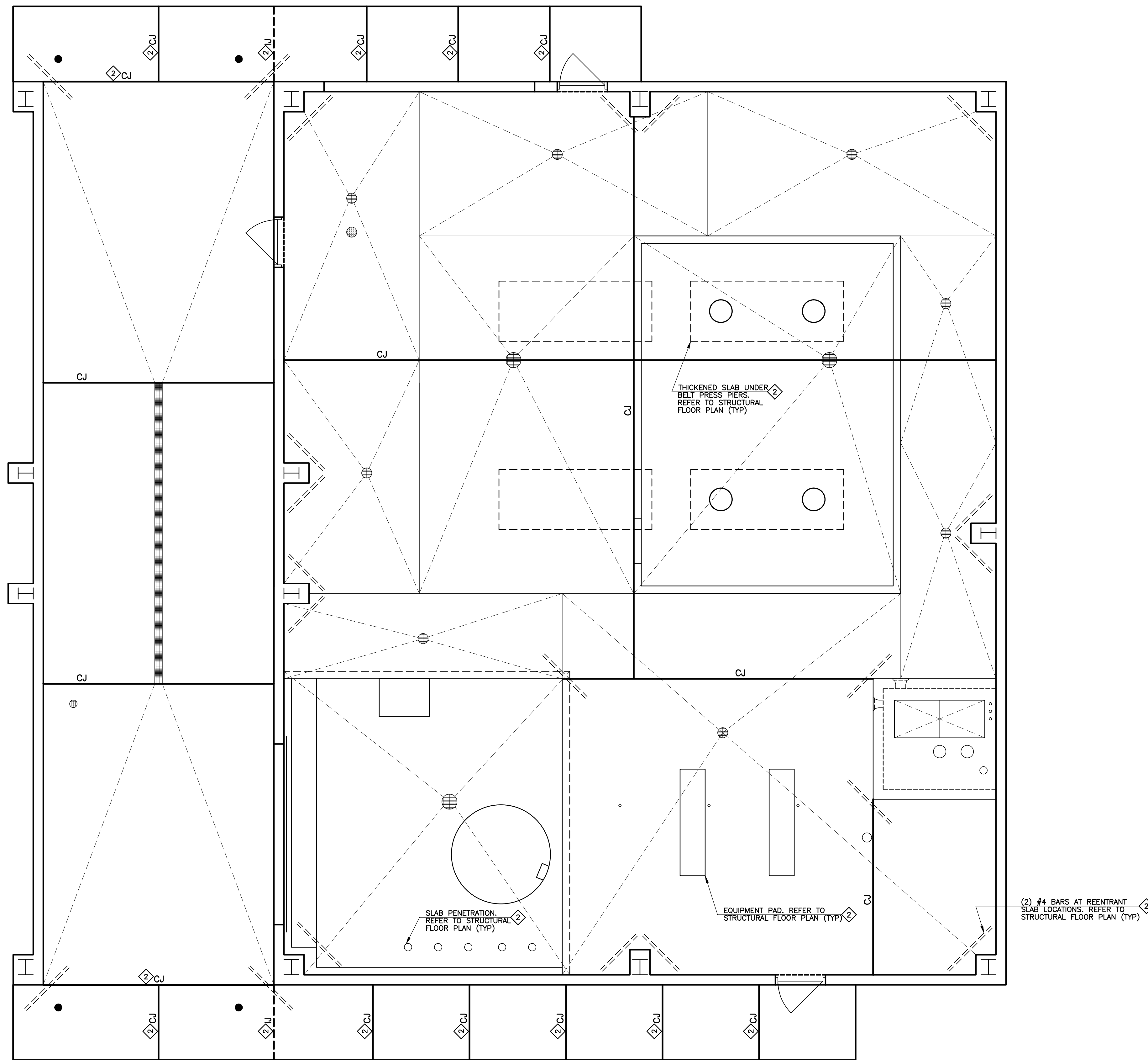
1 JOINTING PLAN BH-4A SCALE: 1/4" = 1'-0"
