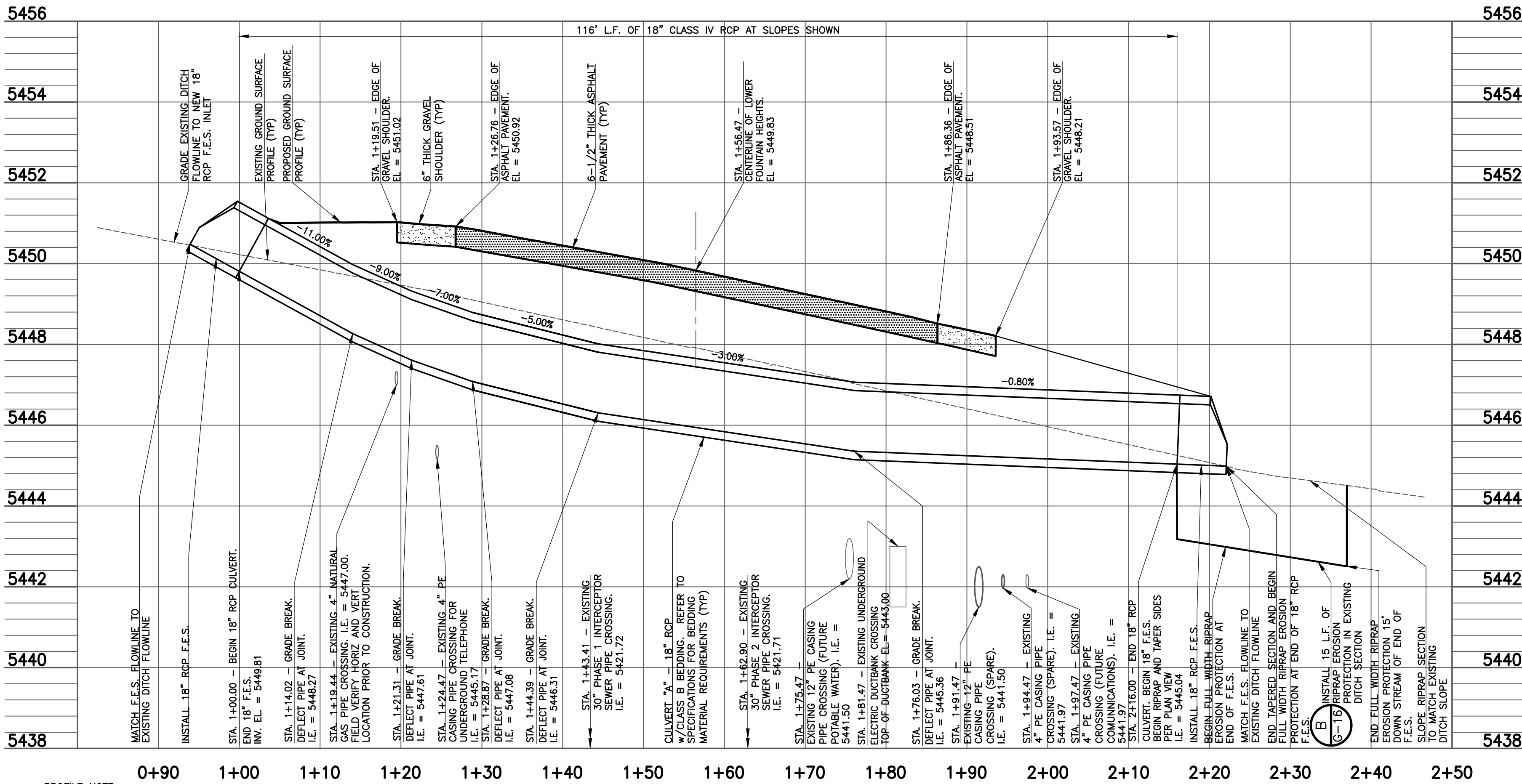
1 CULVERT "A" PLAN VIEW SCALE: 1" = 10'
