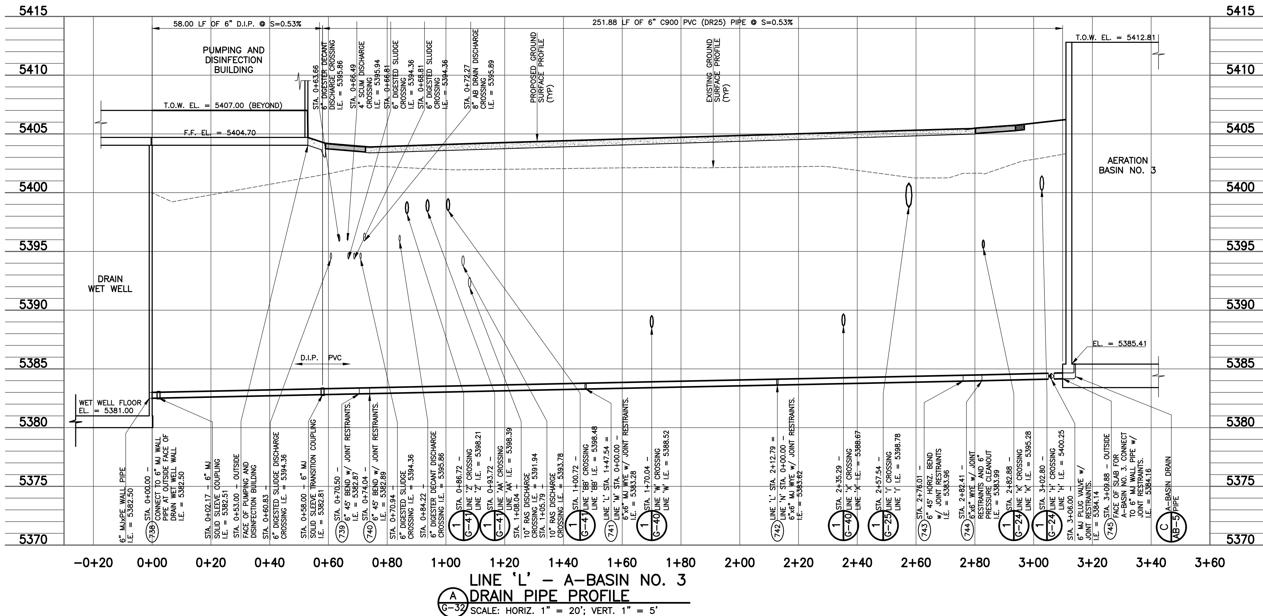
LINE 'L', 'M' AND 'N' A-BASIN DRAIN PIPES PLAN SCALE: 1" = 20'
