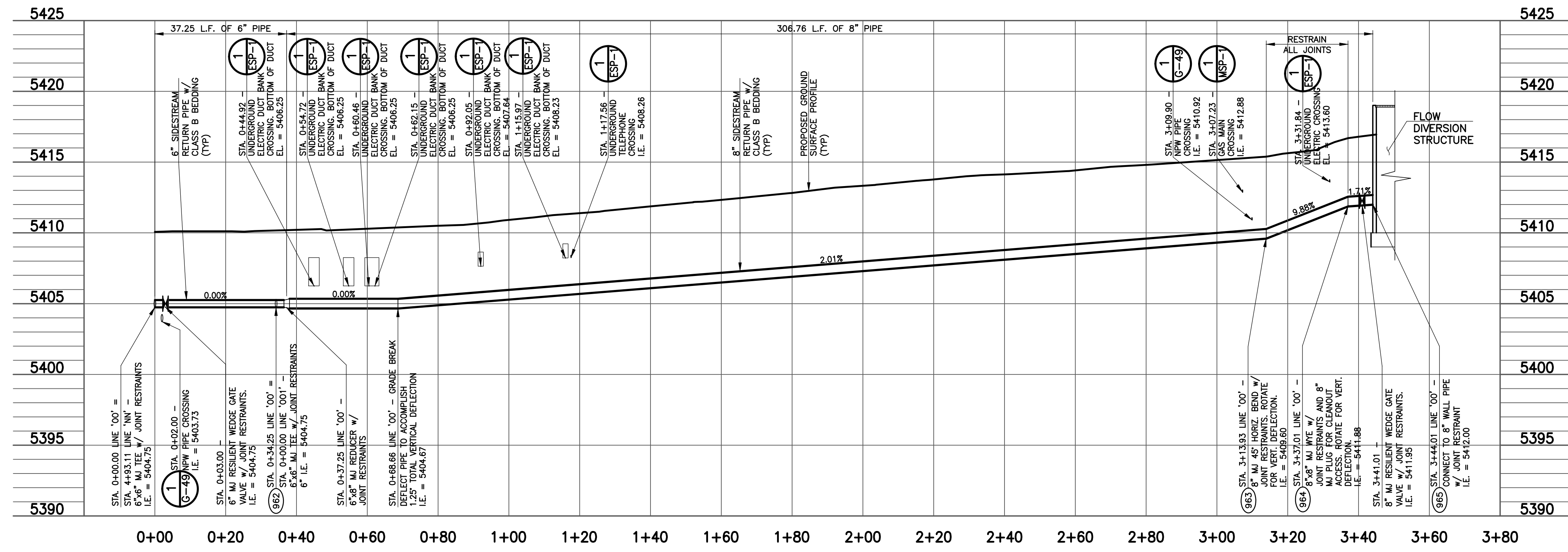
A LINE '00' - SIDESTREAM RETURN PIPE PROFILE SCALE: HORIZ. 1" = 20' VERT. 1" = 5'
