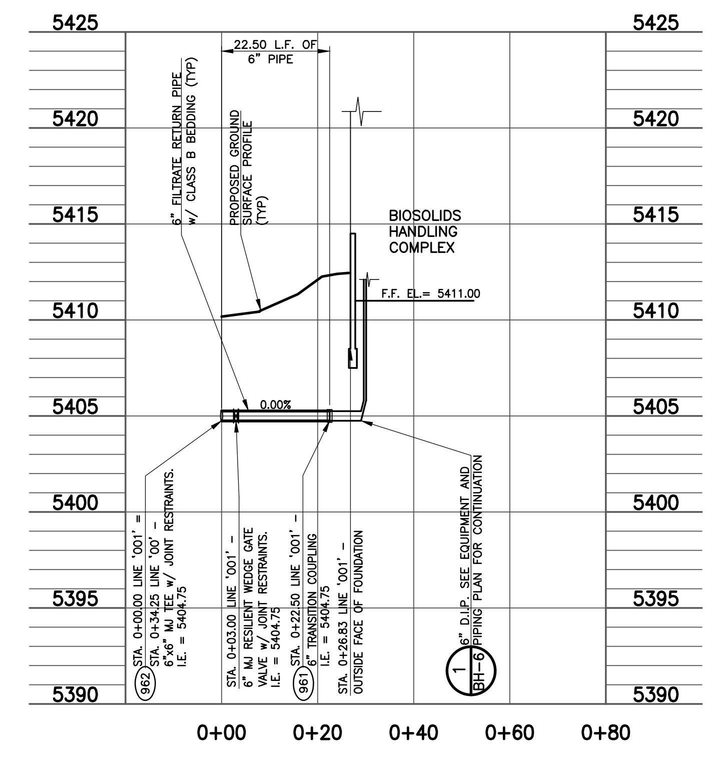
B LINE '00' - FILTRATE RETURN PIPE PROFILE SCALE: HORIZ. 1" = 20' VERT. 1" = 5'
