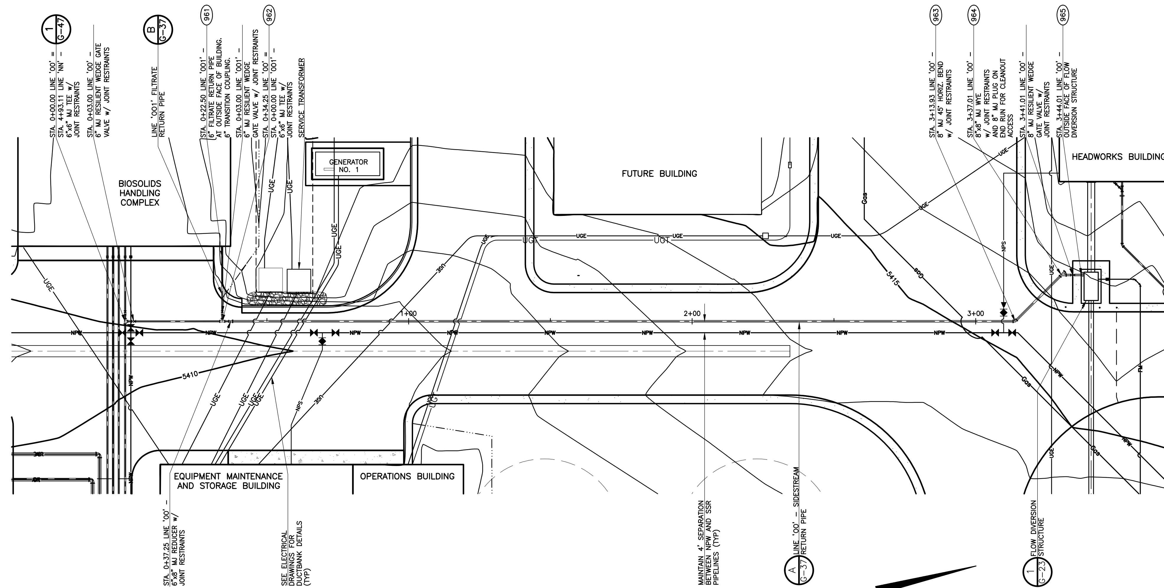
1 LINE '00' PLAN - SIDESTREAM RETURN PIPE PLAN SCALE: 1" = 20'
