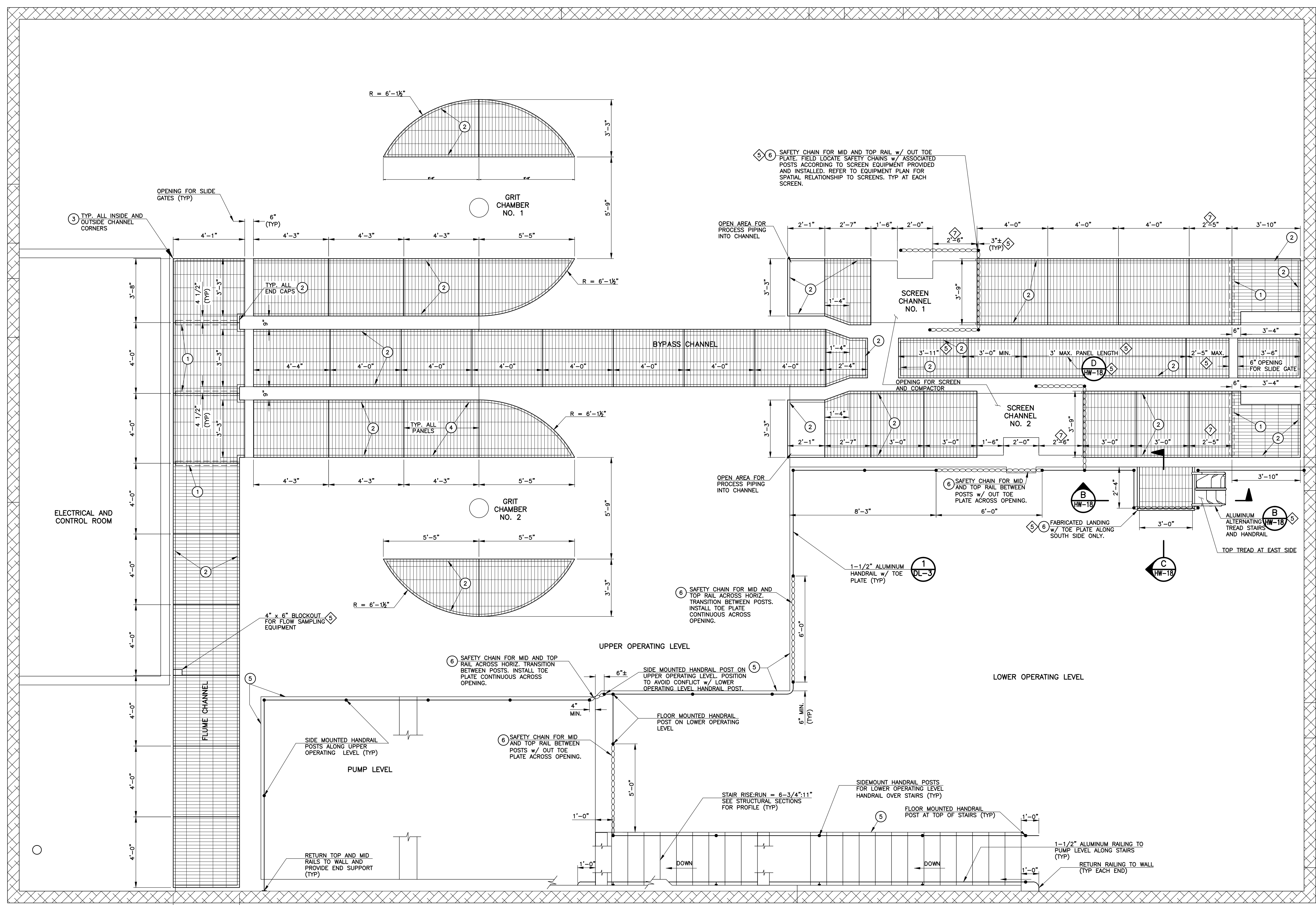
1 GRATING AND HANDRAIL PLAN HW-19 SCALE: 3/8" = 1'-0"
