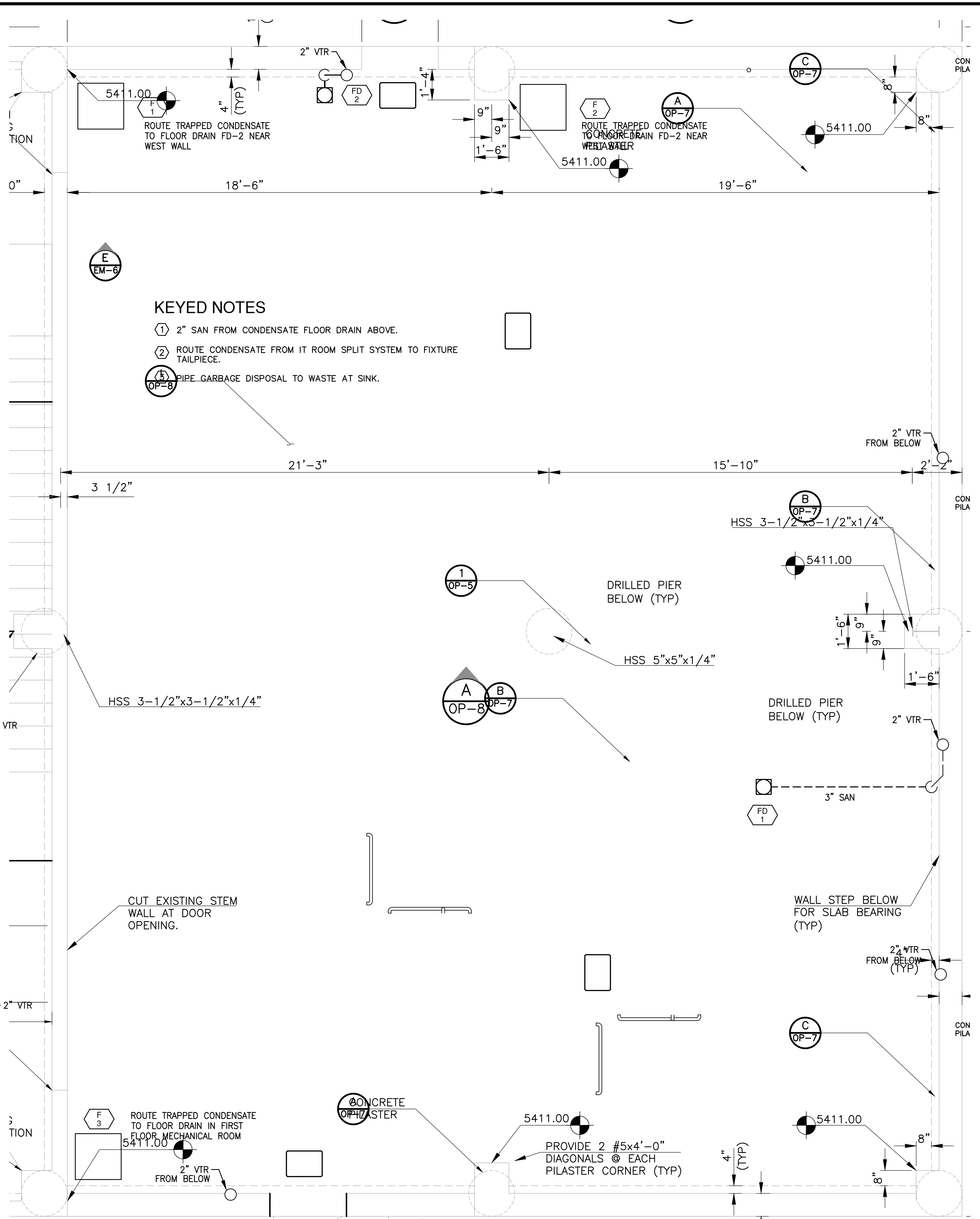
2 PLUMBING SANITARY AND VENT PLAN-UPPER FLOOR POP-P3 SCALE: 3/8" = 1'-0"
