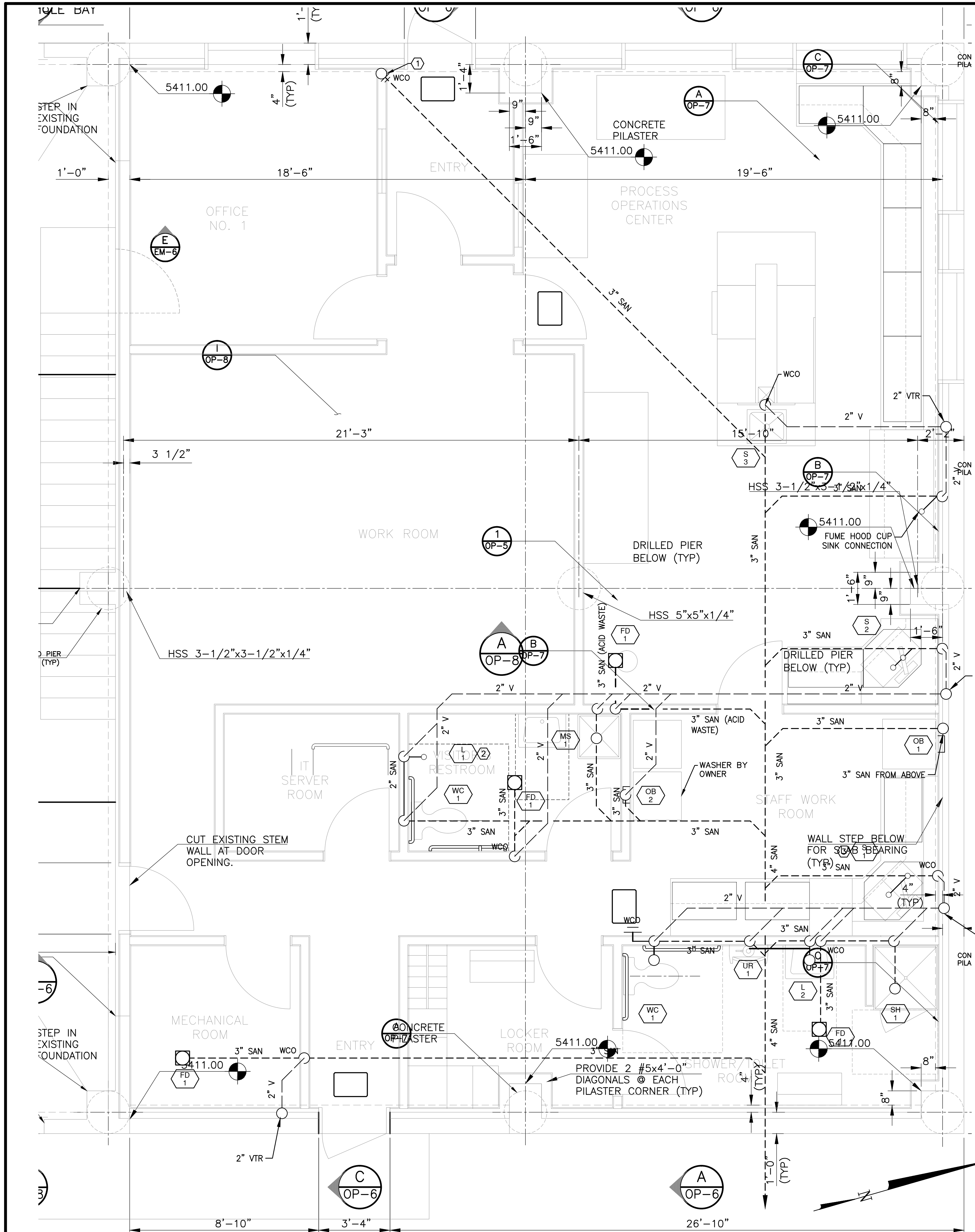
1 PLUMBING SANITARY AND VENT PLAN-LOWER FLOOR POP-P3 SCALE: 3/8" = 1'-0"
