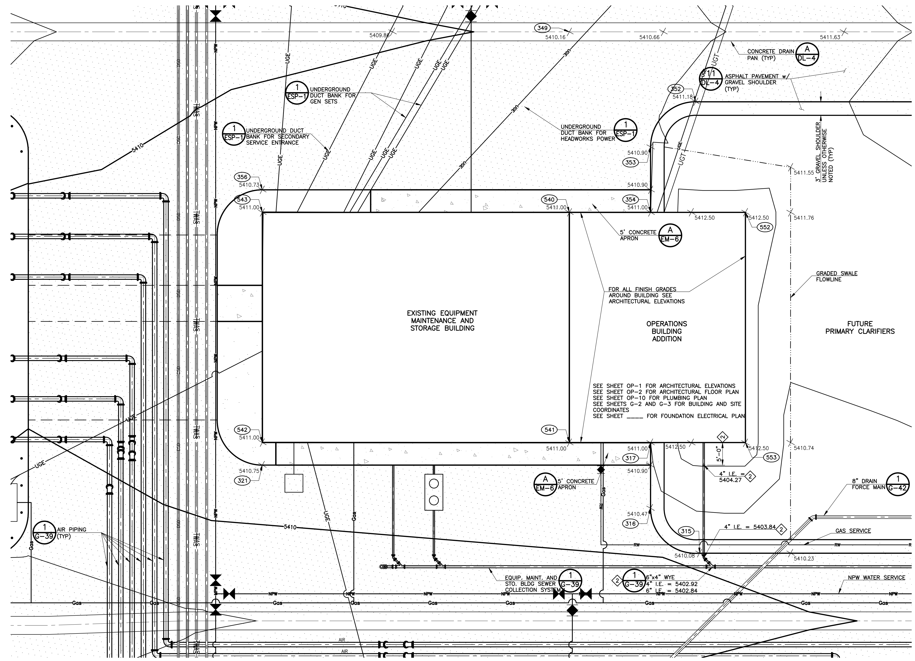
1 OPERATIONS BUILDING DETAILED SITE PLAN OP-9 SCALE: 1" = 10'
