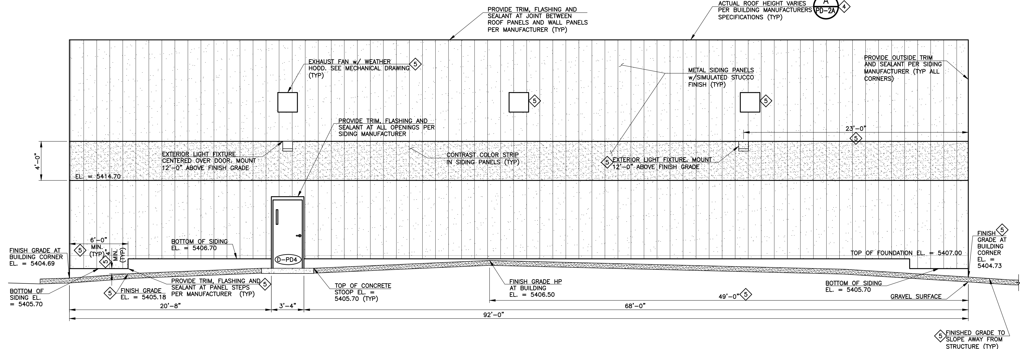
4 PUMPING AND DISINFECTION BUILDING - NORTH ELEVATION SCALE: 1" = 5'-0"
