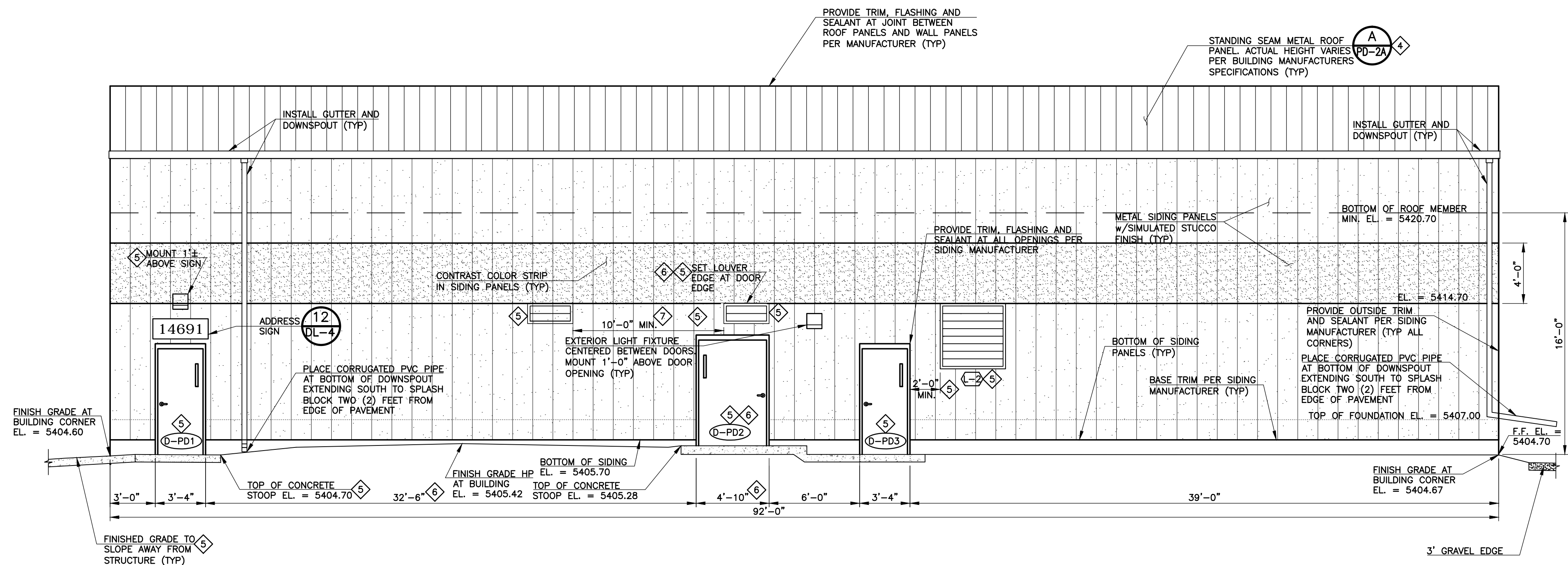
2 PUMPING AND DISINFECTION BUILDING - SOUTH ELEVATION SCALE: 1" = 5'-0"
