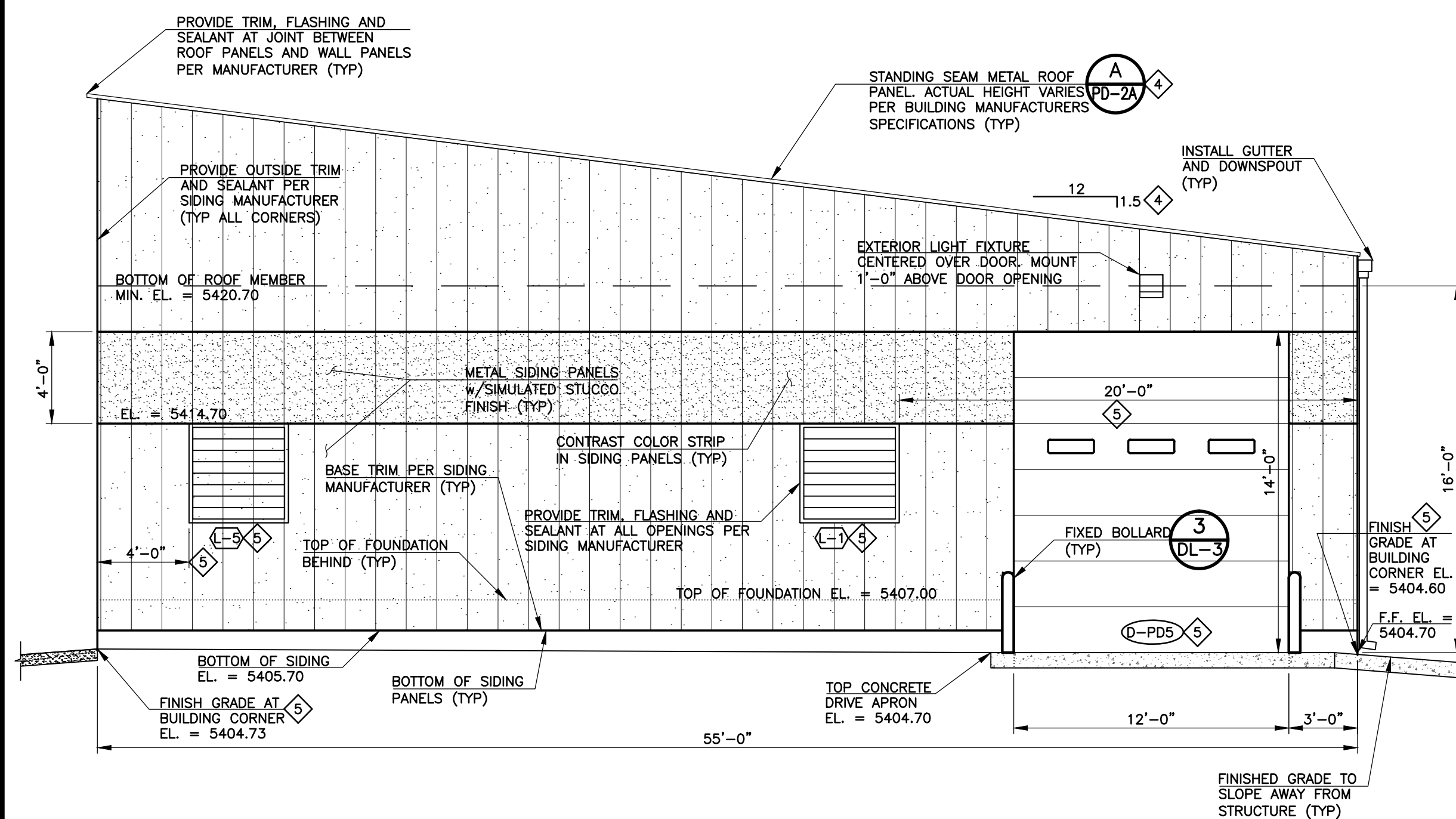
3 PUMPING AND DISINFECTION BUILDING - WEST ELEVATION SCALE: 1" = 5'-0"
