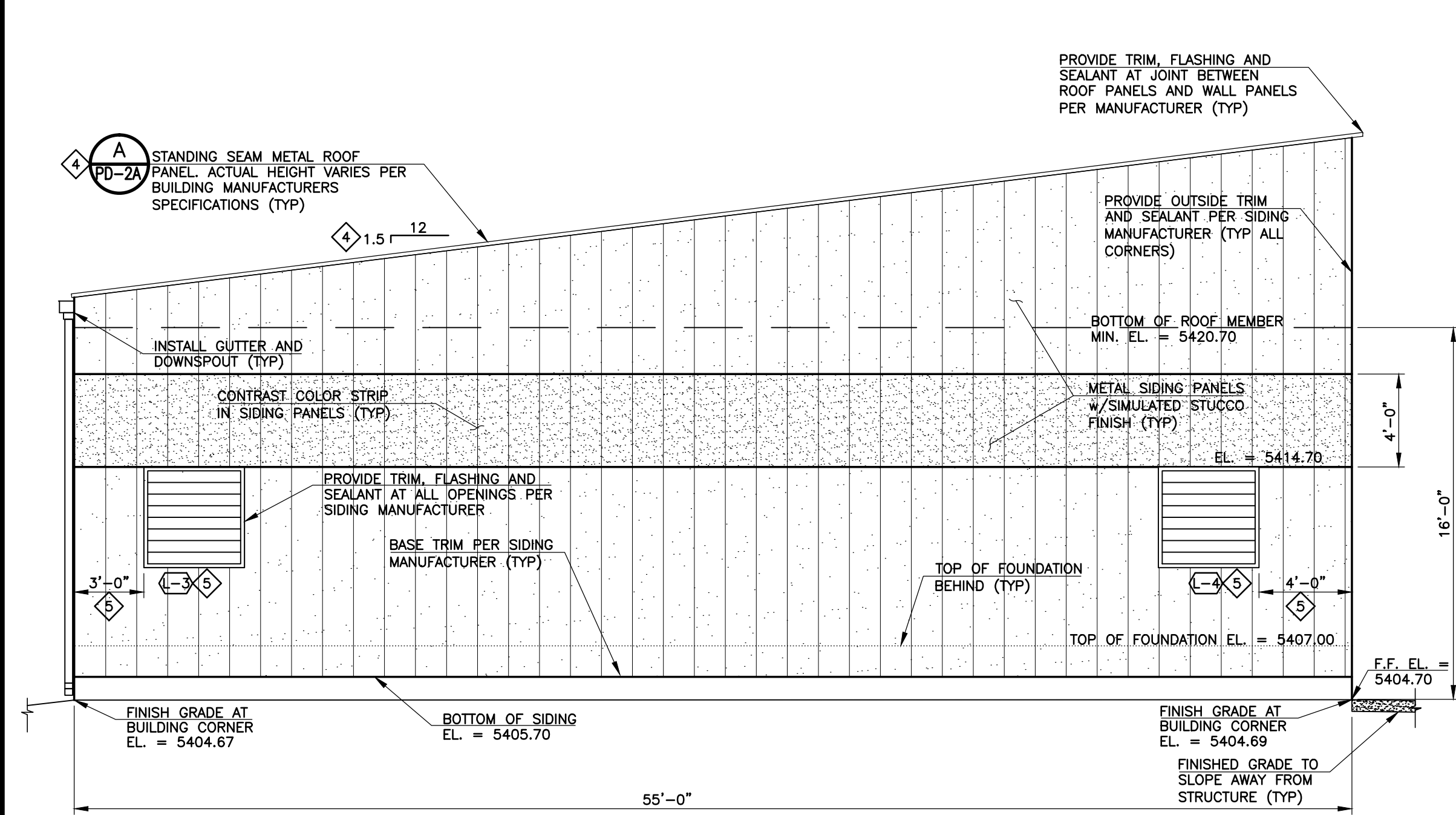
1 PUMPING AND DISINFECTION BUILDING - EAST ELEVATION SCALE: 1" = 5'-0"
