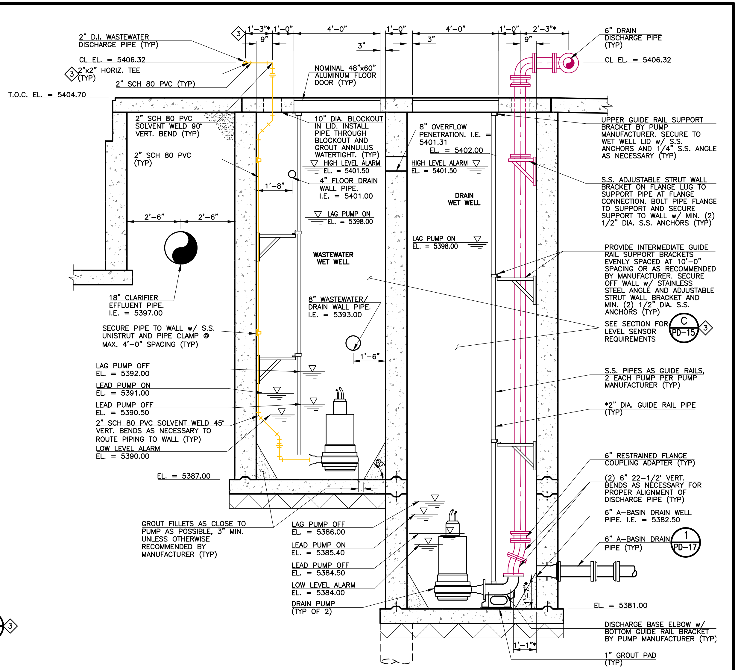
C SECTION PD-17 SCALE: 1/2" = 1'-0"
