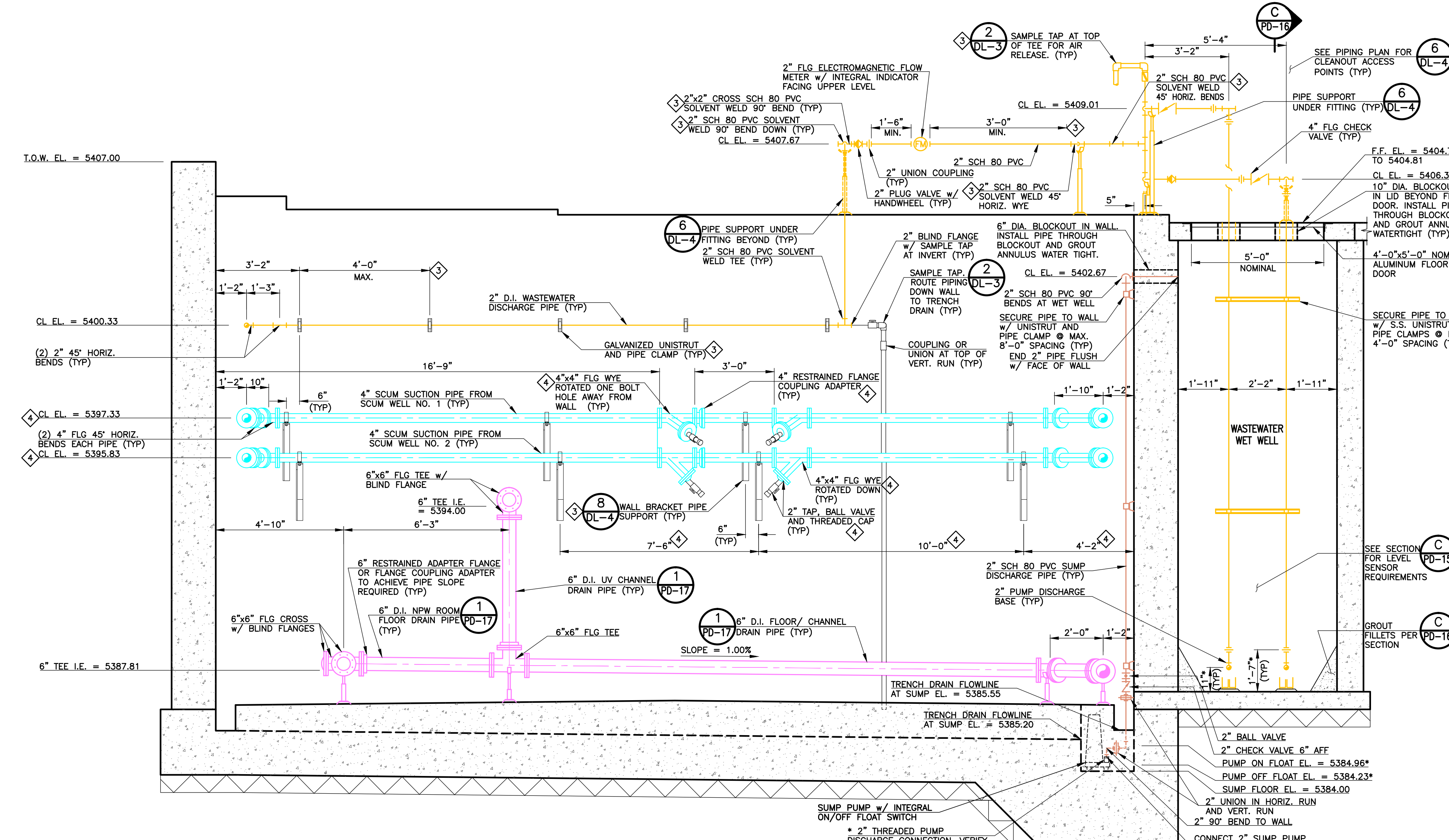
B EAST WALL PROCESS PIPING SECTION PD-16 SCALE: 3/8" = 1'-0"
