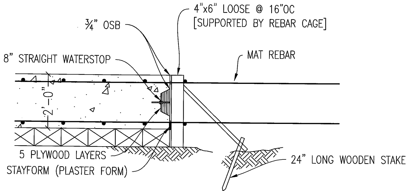
1 MAT SLAB CONSTRUCTION JOINT DETAIL Scale: 1/2"=1'-0"
